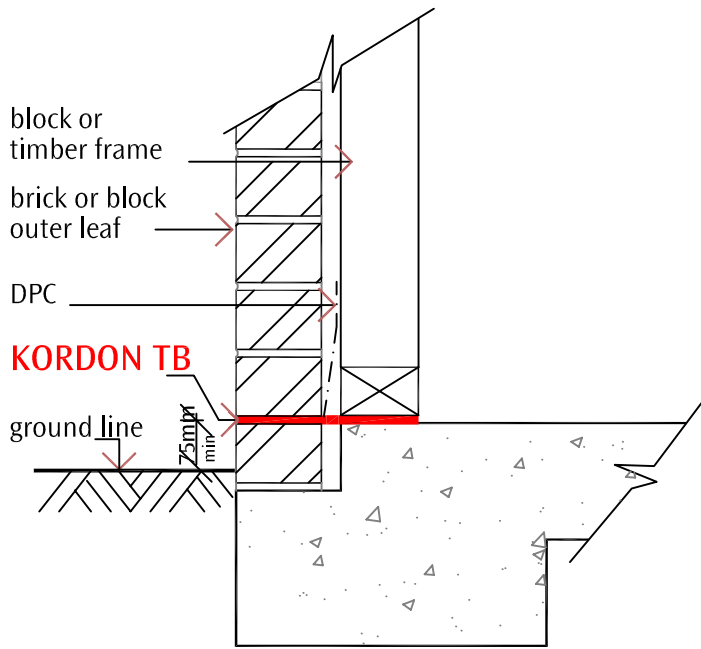
section detail 1
