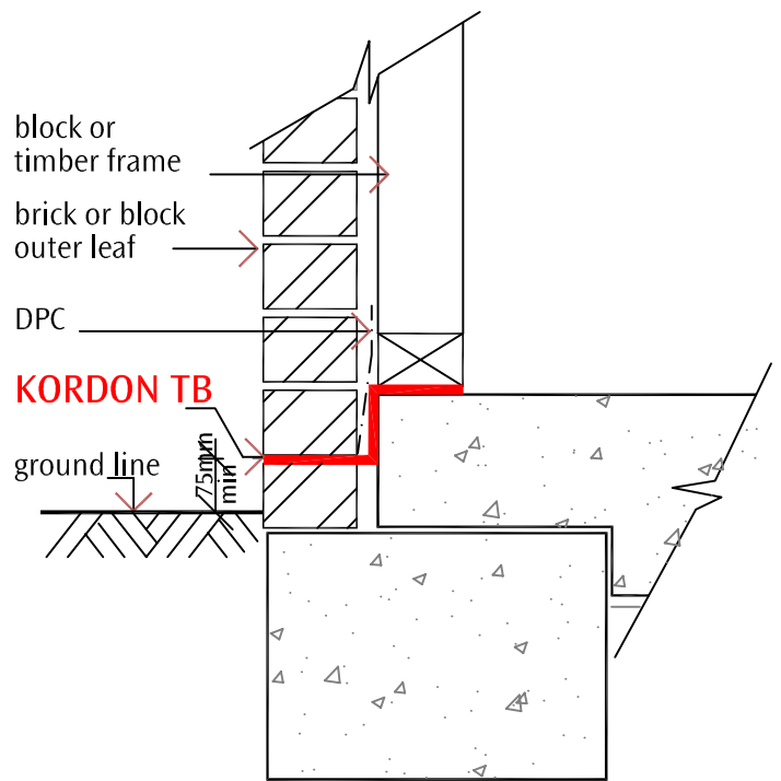
section detail 2
