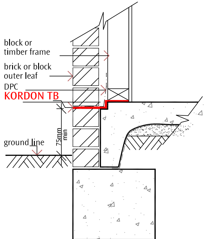
section detail 4
